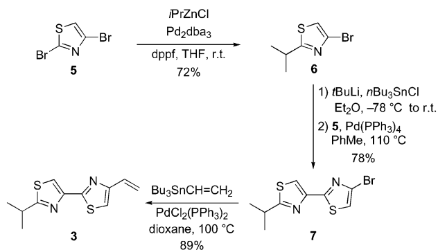
Scheme 2. Synthesis of the vinylbithiazole 3 .
