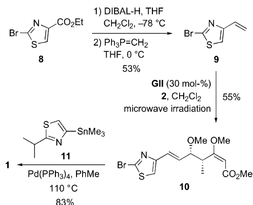
Scheme 4. Synthesis of 1 by sequential CM/Stille coupling.
