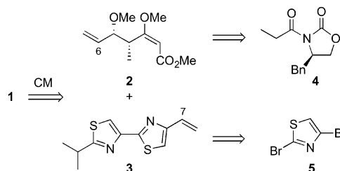
Scheme 1. Retrosynthetic analysis of 1 .
