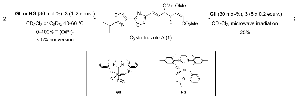
Scheme 3. Synthesis of 1 by CM of 2 and 3 .
